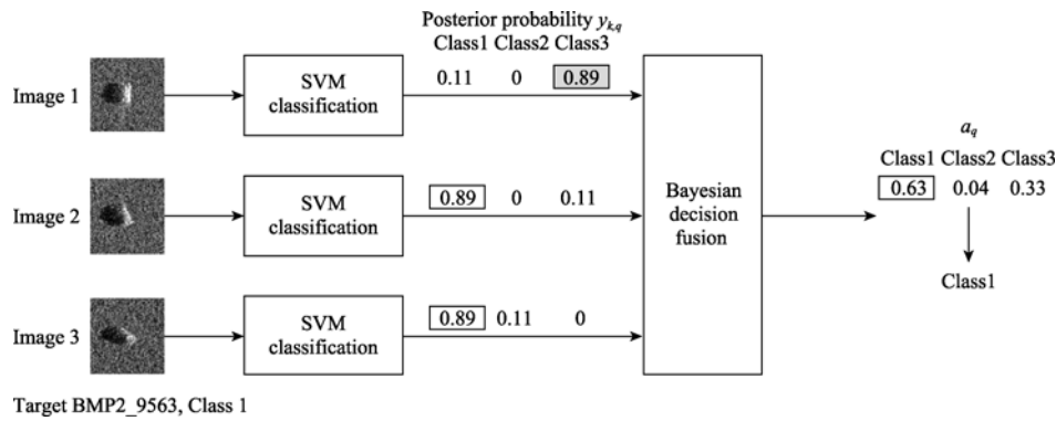
Fig. 6 Bayesian decision fusion process
