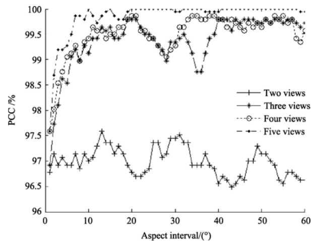
Fig. 7 Probability of correct classification for multiple views decision fusion
