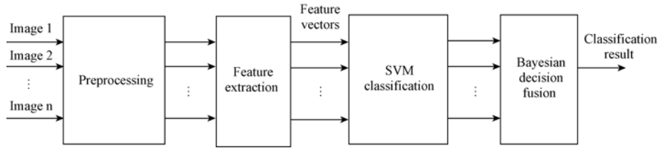
Fig. 1 Process diagram of SAR image target recognition
